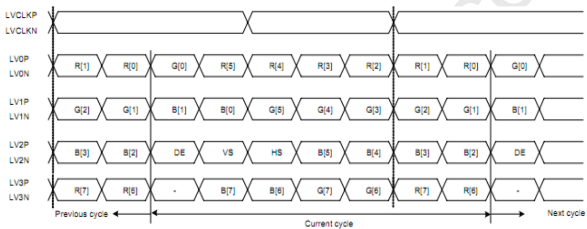
8-bit LVDS input data mapping
