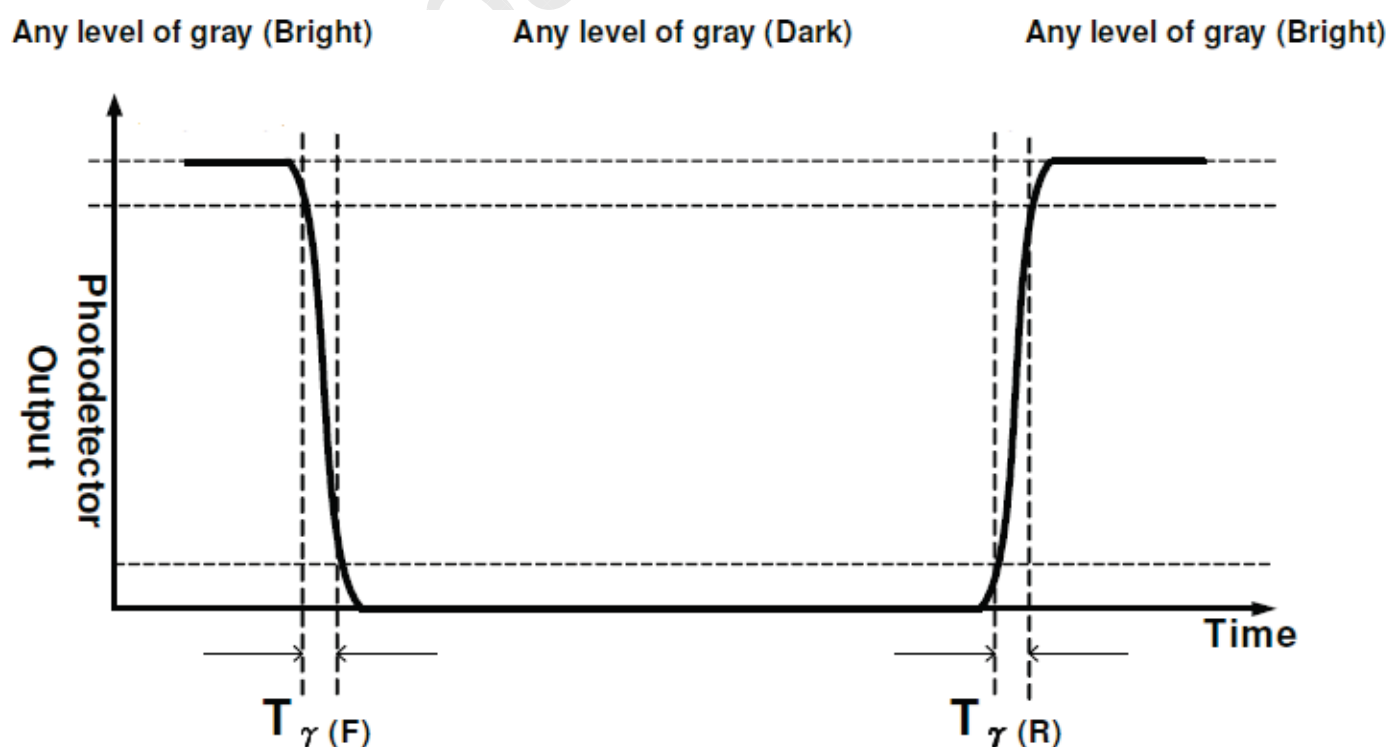
< Figure 3. Response Time Testing >
