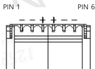
Figure.1 Top view of LED Bar Connector
