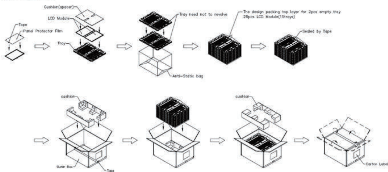
Figure. 9-1 Packing method
