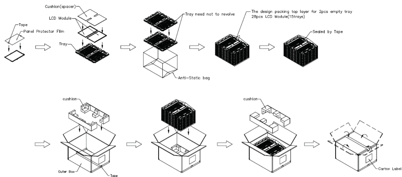
Figure. 9-1 Packing method
