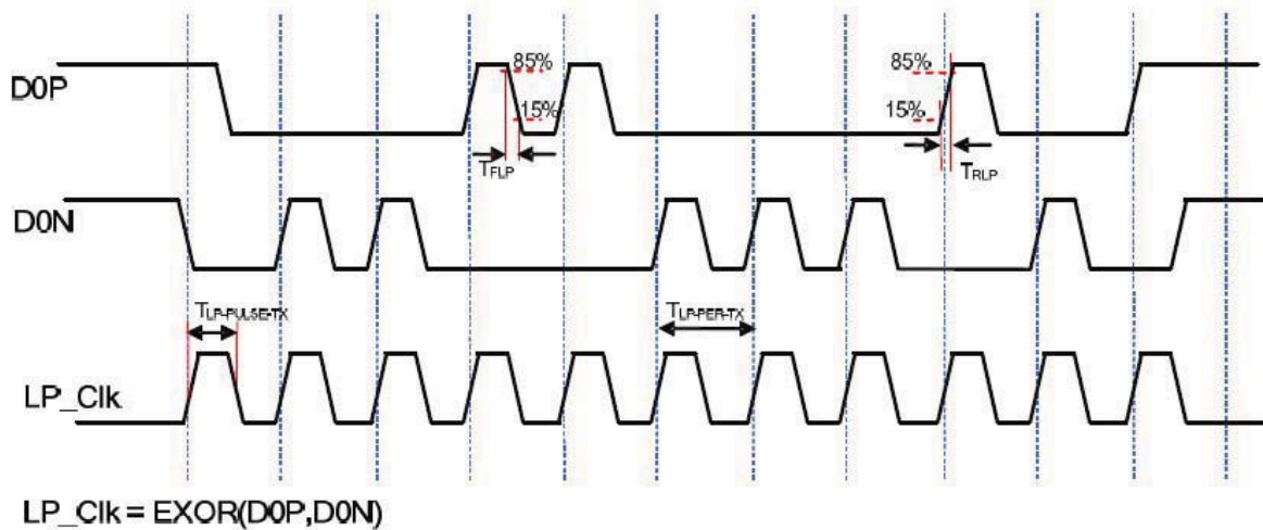
Figure: LP Transmitter Timing Definitions
