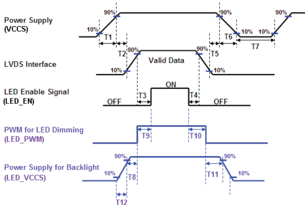
Power ON/OFF sequence timing
