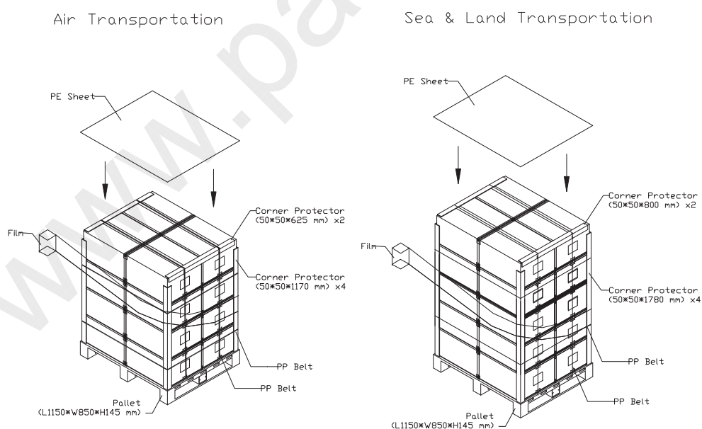
Figure. 6-2 Packing method
