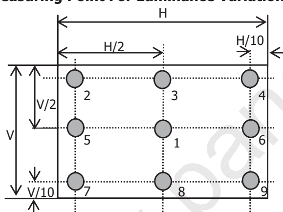
FIG.4-2 Measure Point for Luminance
