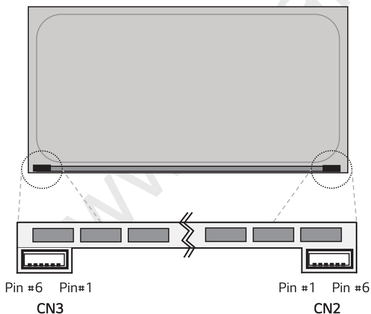
[FIG. 5] Backlight connector view
