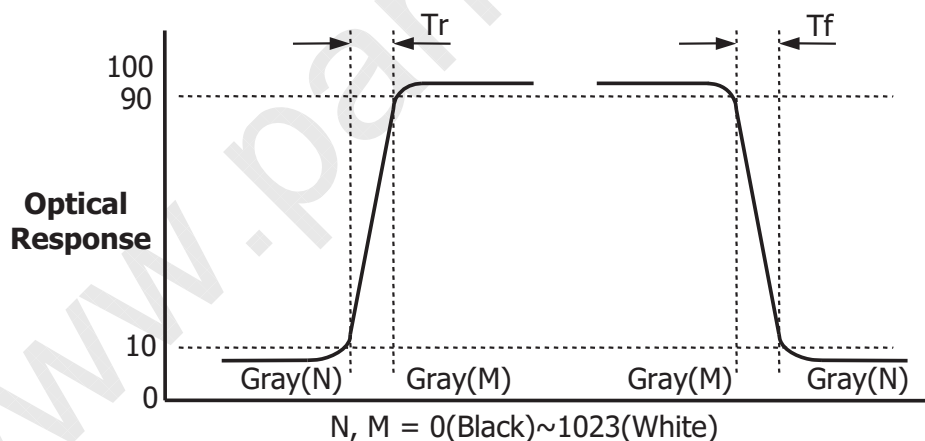
FIG.4-3 Response Time
