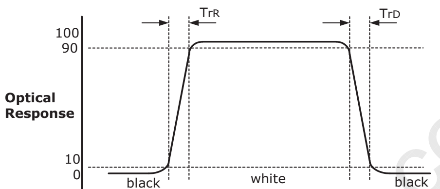
FIG.9 Response time
