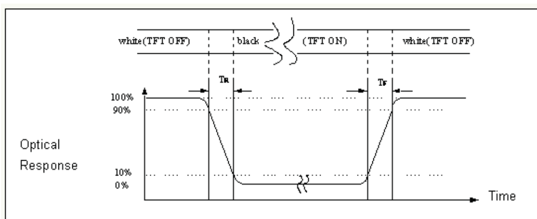
Figure 5 Definition of Response Time
