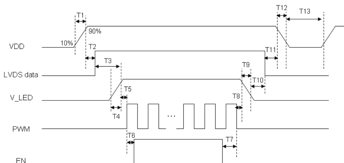
Figure 12 Power Sequence
