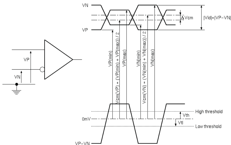
Figure 7 Voltage Definitions
