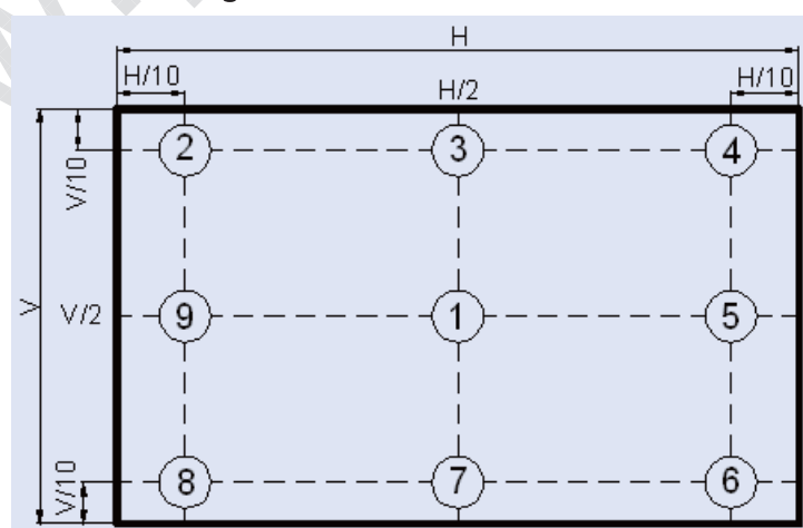
Figure 6 Measurement Locations
