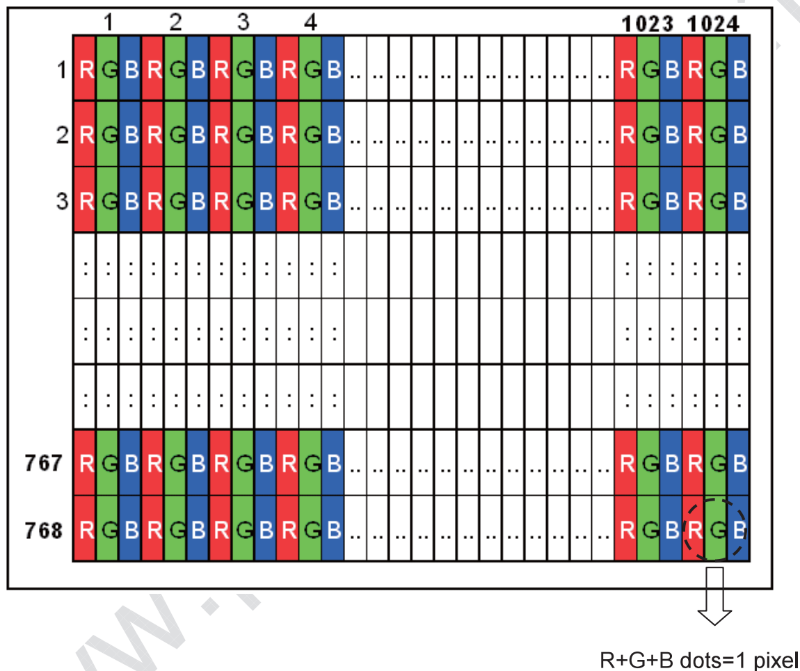
Figure 2 Pixel Format
