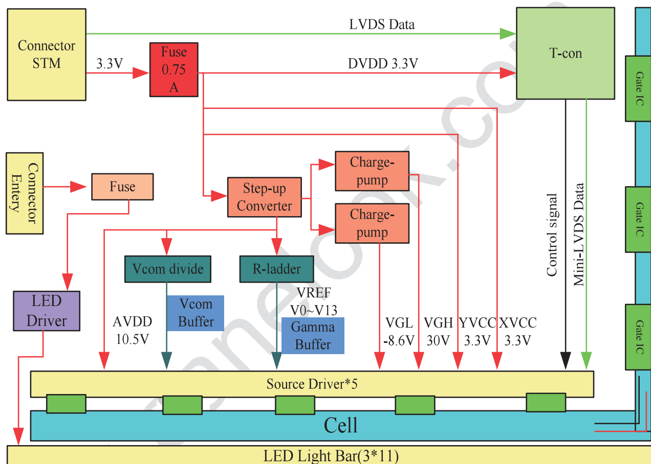
Figure 1 Block Diagram
