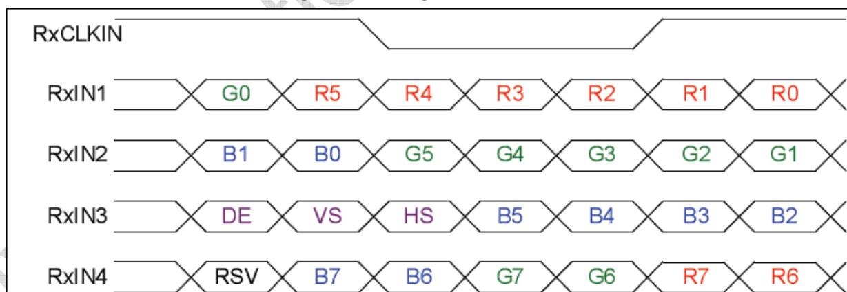
Figure 8 Timing Characteristics
