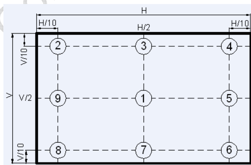
Figure 6 Measurement Locations
