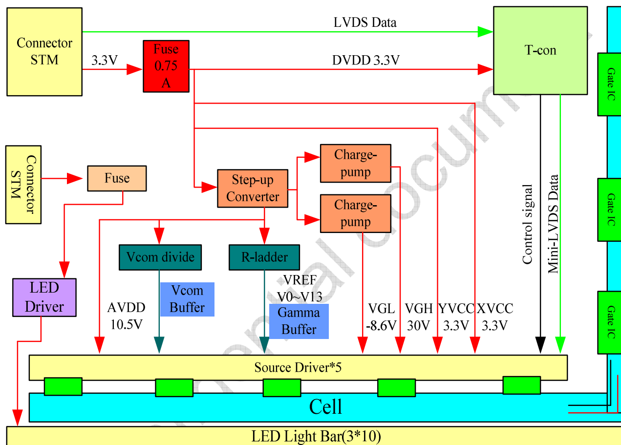
Figure 1 Block Diagram
