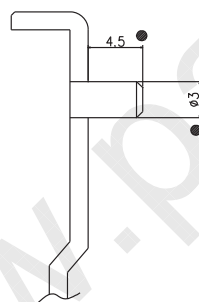
Section B-B (S: 5/1) Total 9pcs "b"
