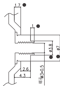
Section D-D (S: 5/1) Total 3pcs "d"
