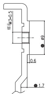
SECTION A-A (Scale: 5/1) Total 9pcs "a"
