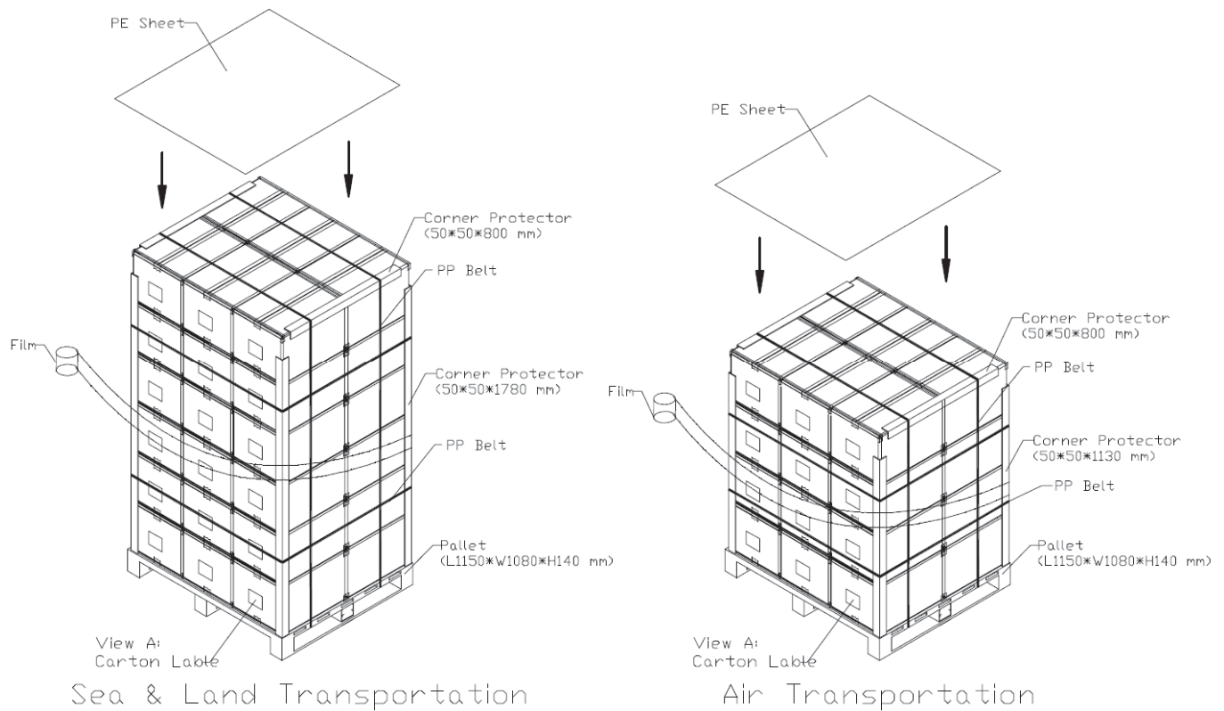
Figure. 7-3 Packing method
