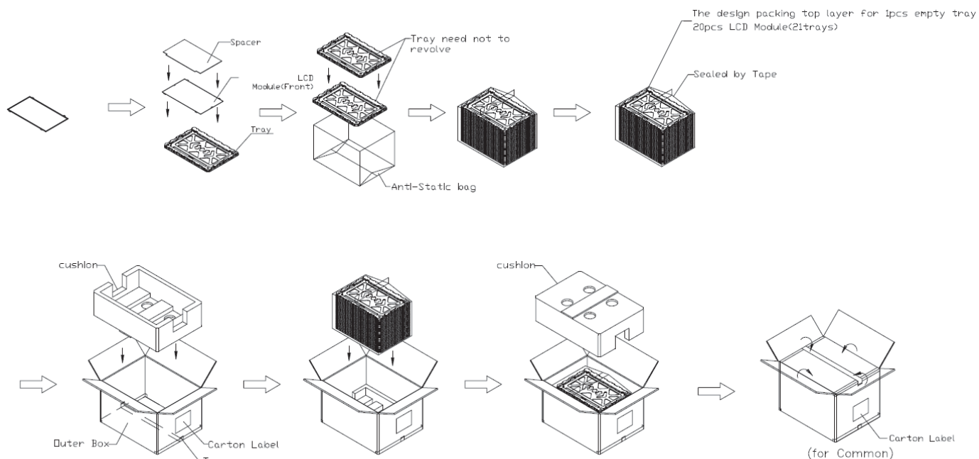
Figure. 7-2 Packing method
