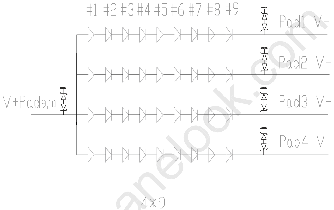
Figure 6. LED Structure
