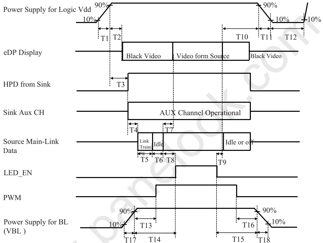
Figure 15. Power Sequence
