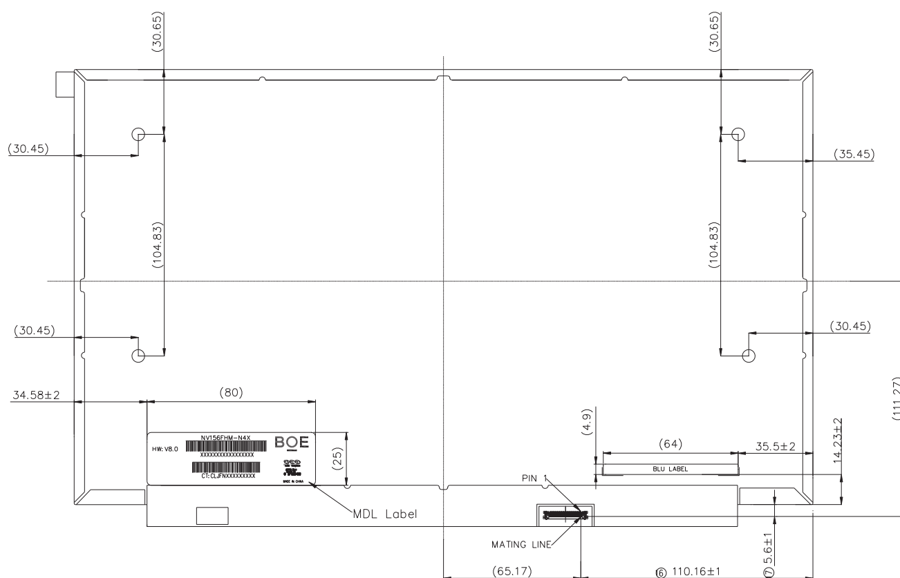
Figure 25. TFT-LCD Module Outline Dimensions (Rear view)
