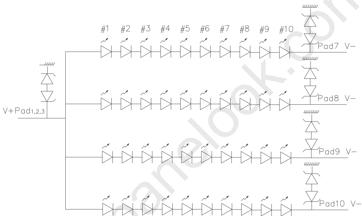
Figure 6. LED Structure
