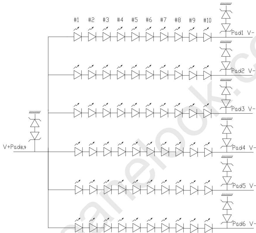
Figure 6. LED Structure
