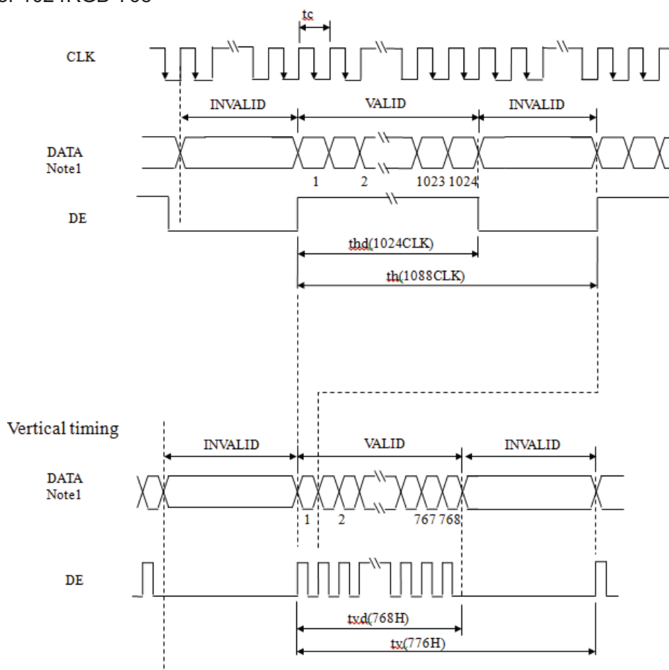
Figure5.1.2 Recommended input timing of LVDS transmitter
