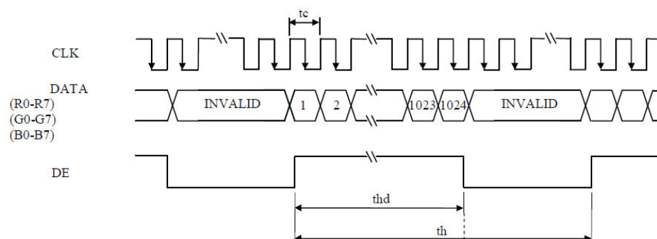
Horizontal timing
